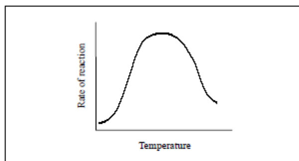
Fig 2. Effect of temperature on enzyme activity
